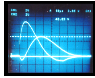
Center Conductor "Surge" Delay can damage equipment
