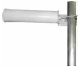
TerraWave 5.8 GHz 15 dBi Yagi Antenna TESSCO # 484982
